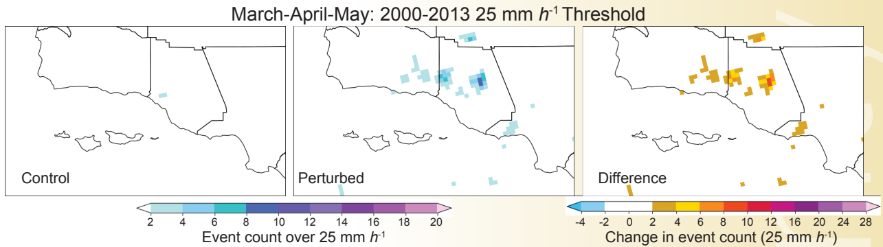
FIGURE 4.16: Number of >25 mm h^{-1} events summed over March–April–May periods in the 2000–2013 period for a) control simulation b) perturbed simulation and c) difference between b and a (perturbed minus control).
