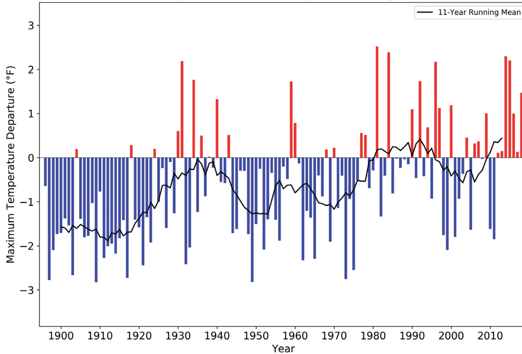
FIGURE 1.2: Maximum temperature departure from 1981–2010 average for 1 October–30 September (Water Year) periods for Water Years 1896 through 2018 for the South Coast climate region of California. Source: California Climate Tracker https://wrcc.dri.edu/Climate/Tracker/CA/
