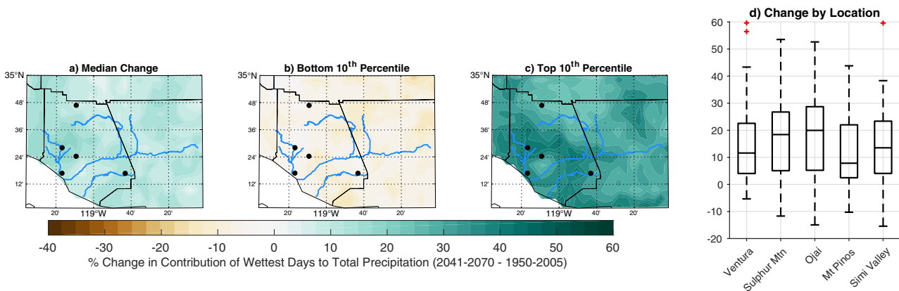
FIGURE A.14: Changes in contribution of the top 5% of wettest days to total annual precipitation (2041–2070 minus 1950–2005) as: a) Median change in contribution across models; b) The bottom 10 th percentile (decile with smallest or negative change in contribution) in a distribution fit to the model range of values; c) The top 10 th percentile (decile with greatest positive changes in contribution) in a distribution fit to the model range of values; d) Spread in change in contribution across all 32 CMIP5 models for five selected locations within Ventura County (black dots on map).
