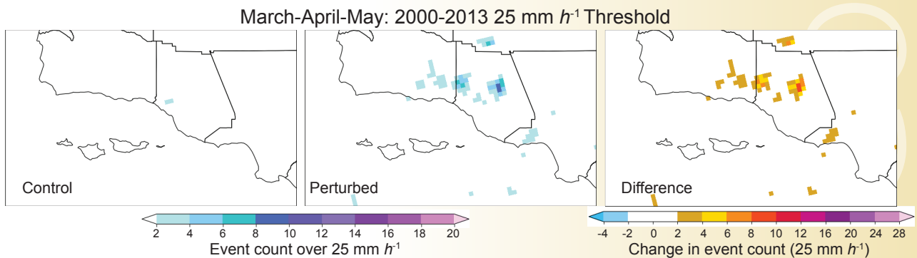
FIGURE 4.12: Number of >25 \text{ mm } h^{-1} events summed over March–April–May periods in the 2000–2013 period for a) control simulation b) perturbed simulation and c) difference between b and a (perturbed minus control).
