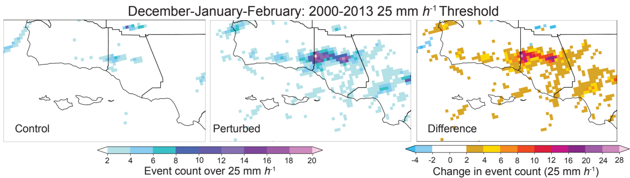
FIGURE 4.15: Number of >25 mm h^{-1} events summed over December–January–February periods in the 2000–2013 period for a) control simulation b) perturbed simulation and c) difference between b and a (perturbed minus control).
