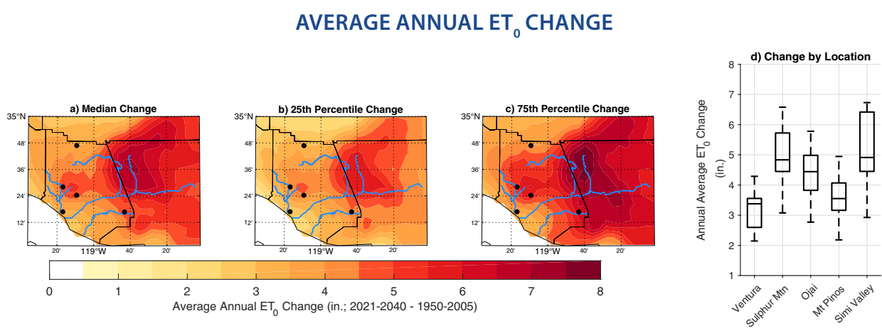
FIGURE 5.1: Change in average annual reference evapotranspiration ( ET_0 ), 2021–2040 mean minus 1950–2005 mean for the a) median change in ET_0 ; b) 25 th percentile (bottom quartile) change in ET_0 ; c) 75 th percentile (upper quartile) change in ET_0 ; d) Spread in change of average annual ET_0 for five selected locations within Ventura County (black dots on map).
