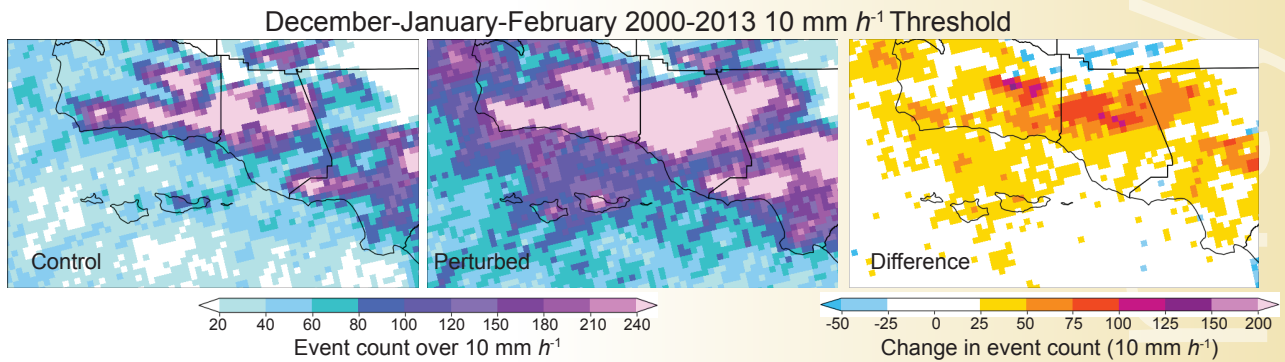
FIGURE 4.11: Number of >10 \text{ mm } h^{-1} events summed over December–January–February periods in the 2000–2013 period for a) control simulation b) perturbed simulation and c) difference between b and a (perturbed minus control).
