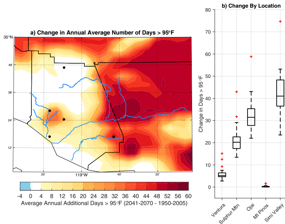
FIGURE A.5: Change in average annual number of days with maximum temperature >95°F, 2041–2070 mean minus 1950–2005 mean. Left panel shows minimum change that ≥75% of models (≥24 of 32) agree on. Right panel depicts spread of change in average annual number of days with maximum temperature >95°F across all 32 CMIP5 models for five selected locations within Ventura County (black dots on map).
