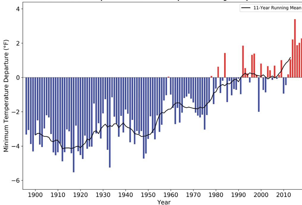
FIGURE 1.3: Minimum temperature departure from 1981–2010 average for 1 October–30 September (Water Year) periods for Water Years 1896 through 2018 for the South Coast climate region of California. Source: California Climate Tracker https://wrcc.dri.edu/Climate/Tracker/CA/
