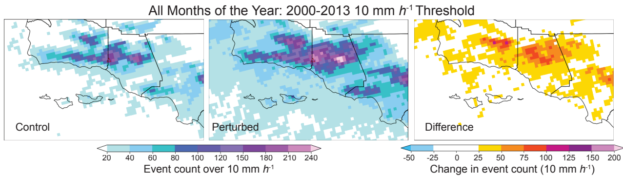
FIGURE 4.10: Number of >10 mm h -1 events summed over all months in the 2000–2013 period for a) control simulation and b) perturbed simulation and c) difference between b) and a) (perturbed minus control).
