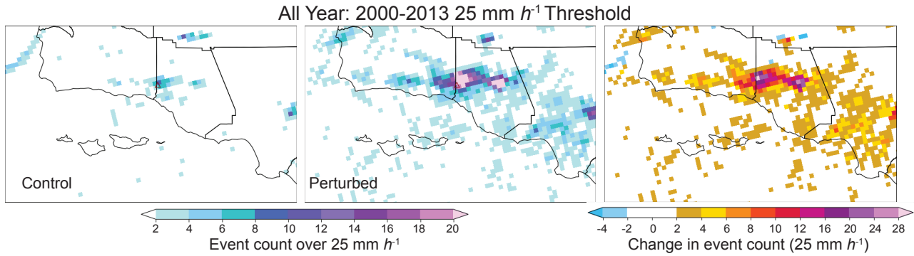
FIGURE 4.14: Number of >25 mm h^{-1} events summed over all months in the 2000–2013 period for a) control simulation and b) perturbed simulation and c) difference between b and a (perturbed minus control).
