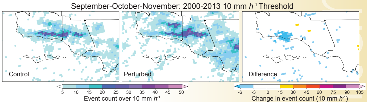
FIGURE 4.13: Number of >10 \text{ mm } h^{-1} events summed over September–October–November periods in the 2000–2013 period for a) control simulation b) perturbed simulation and c) difference between b and a (perturbed minus control).
