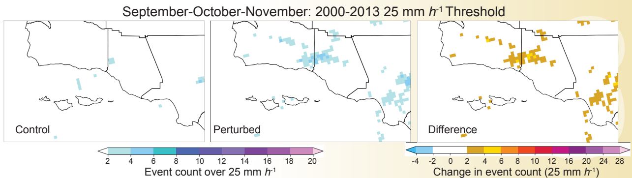
FIGURE 4.17: Number of >25 mm h^{-1} events summed over September–October–November periods in the 2000–2013 period for a) control simulation b) perturbed simulation and c) difference between b and a (perturbed minus control).
