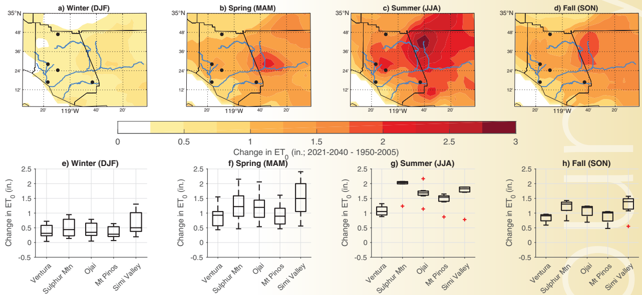
FIGURE 5.2: Change in seasonal average reference evapotranspiration ( ET_0 ), 2021–2040 minus 1950–2005 for winter (a), spring (b), summer (c) and fall (d). Spread in change in seasonal ET_0 across all seven CMIP5 models for five selected locations within Ventura County (black dots on map) for winter (e), spring (f), summer (g) and fall (h).
