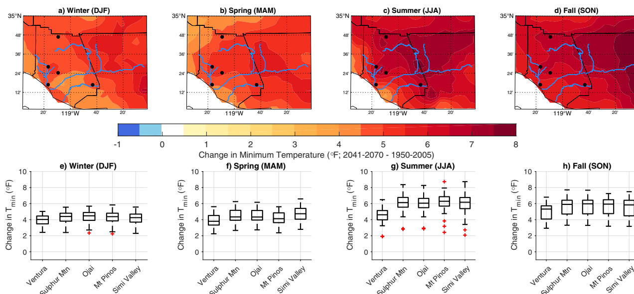
FIGURE A.2: Change in minimum temperature by season, 2041–2070 mean minus 1950–2005 mean. The top row shows the minimum change that ≥75% of models (≥24 of 32) agree on. Bottom row depicts spread of average change in minimum temperatures across all 32 CMIP5 models for five selected locations within Ventura County (black dots on map).
