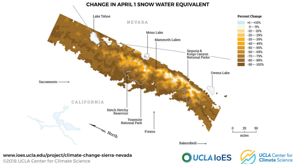
FIGURE 6.1: Business-as-usual snowpack, 2081–2100. This map depicts the percentage of April 1 snow water equivalent projected to be lost over the Sierra Nevada by 2081–2100 under the RCP 8.5 (business-as-usual) scenario compared with the historical period 1981–2000. Source: Reich et al. (2018).
