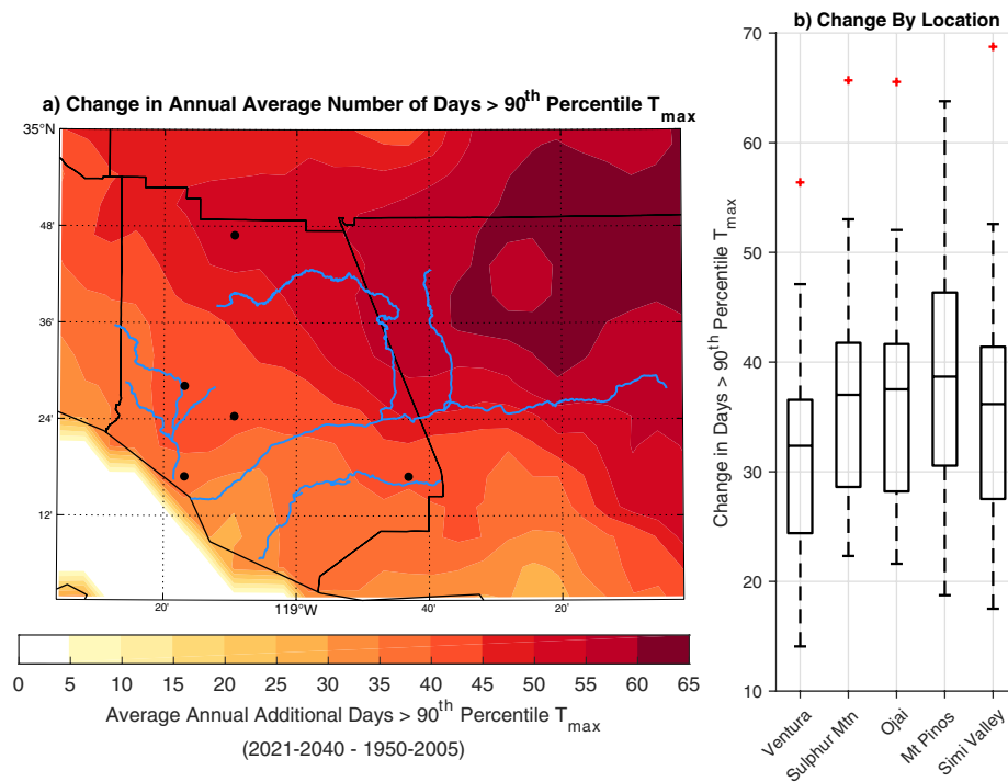
FIGURE 3.7: Change in average annual number of days with maximum temperature exceeding the historic 90 th percentile maximum temperature. Panel a shows minimum change that ≥75% of models (≥24 of 32) agree on. Panel b depicts spread of change in average annual number of days with maximum temperature >90 th percentile across all 32 CMIP5 models for five selected locations within Ventura County (black dots on map).
