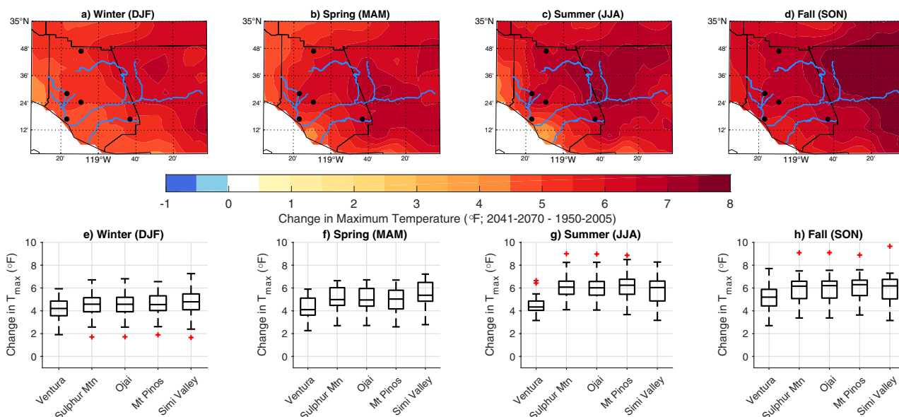
FIGURE A.1: Change in maximum temperature by season, 2041–2070 mean minus 1950–2005 mean. The top row shows the minimum change that ≥75% of models (≥24 of 32) agree on. Bottom row depicts spread of average change in maximum temperatures across all 32 CMIP5 models for five selected locations within Ventura County (black dots on map). Rivers and creeks are shown as blue lines.
