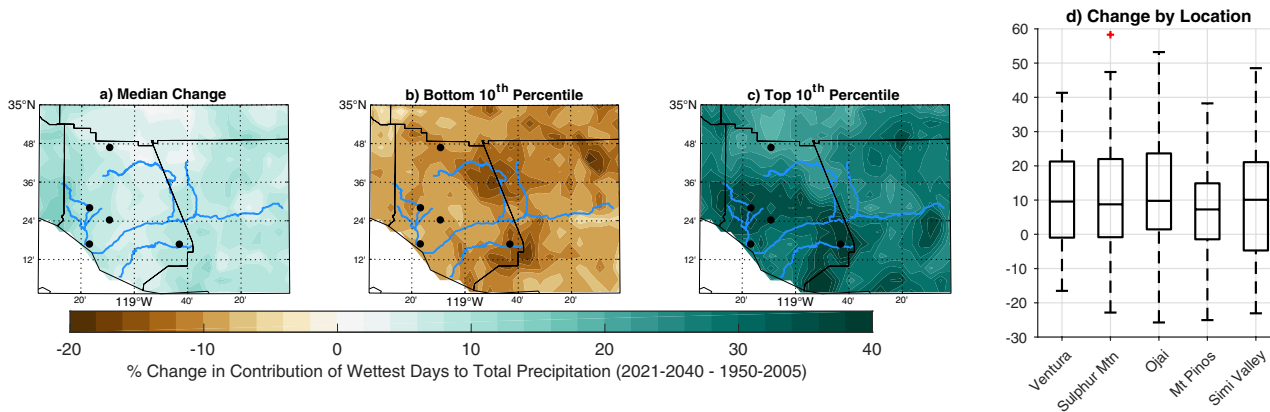
FIGURE 4.4: Changes in contribution of the top 5% of wettest days to total annual precipitation (2021–2040 minus 1950–2005) as: a) Median change in contribution across models; b) The bottom 10 th percentile (decile with smallest or negative change in contribution) in a distribution fit to the model range of values; c) The top 10 th percentile (decile with greatest positive changes in contribution) in a distribution fit to the model range of values; d) Spread in change in contribution across all 32 CMIP5 models for five selected locations within Ventura County (black dots on map).
