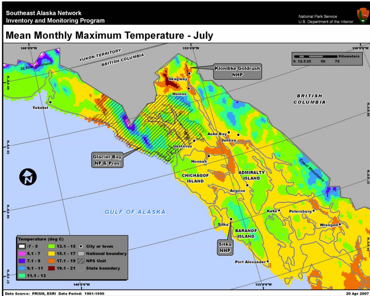
Figure 2.5. Mean July maximum temperature, 1961-1990, for the SEAN.
