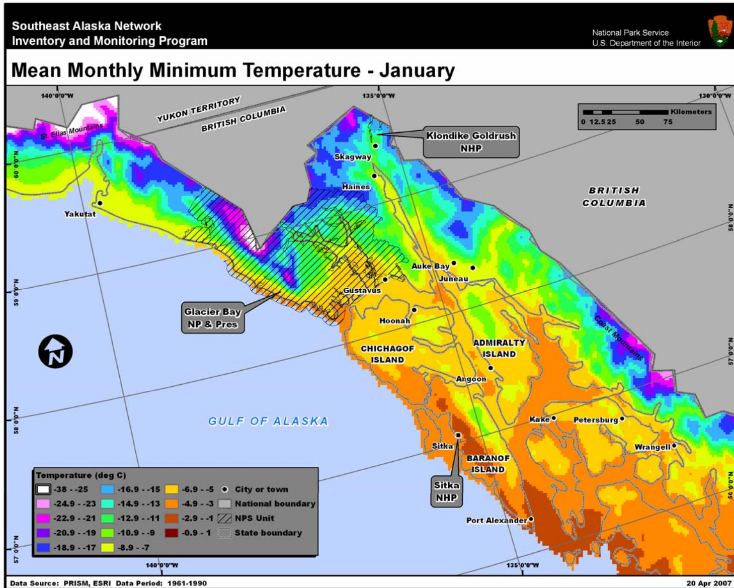
Figure 2.4. Mean January minimum temperature, 1961-1990, for the SEAN.
