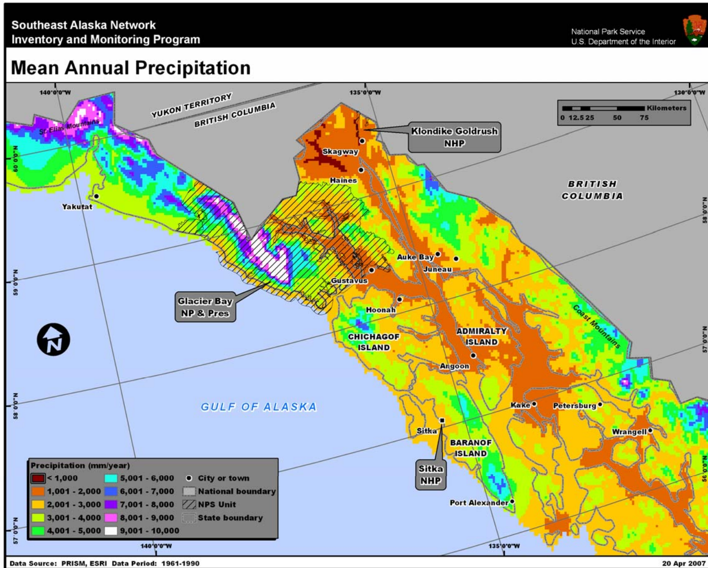
Figure 2.1. Mean annual precipitation, 1961-1990, for the SEAN.
