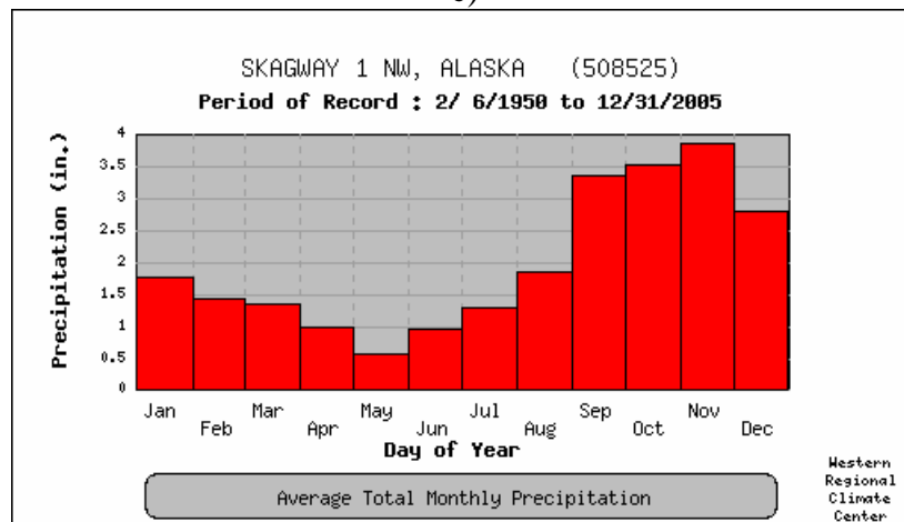
Figure 2.2. Mean monthly precipitation at selected stations in the SEAN. Sitka FAA Japonski AP (a) is near SITK, Gustavus 2 SW (b) is just southeast of GLBA, and Skagway 1 NW (c) is near KLGO.
