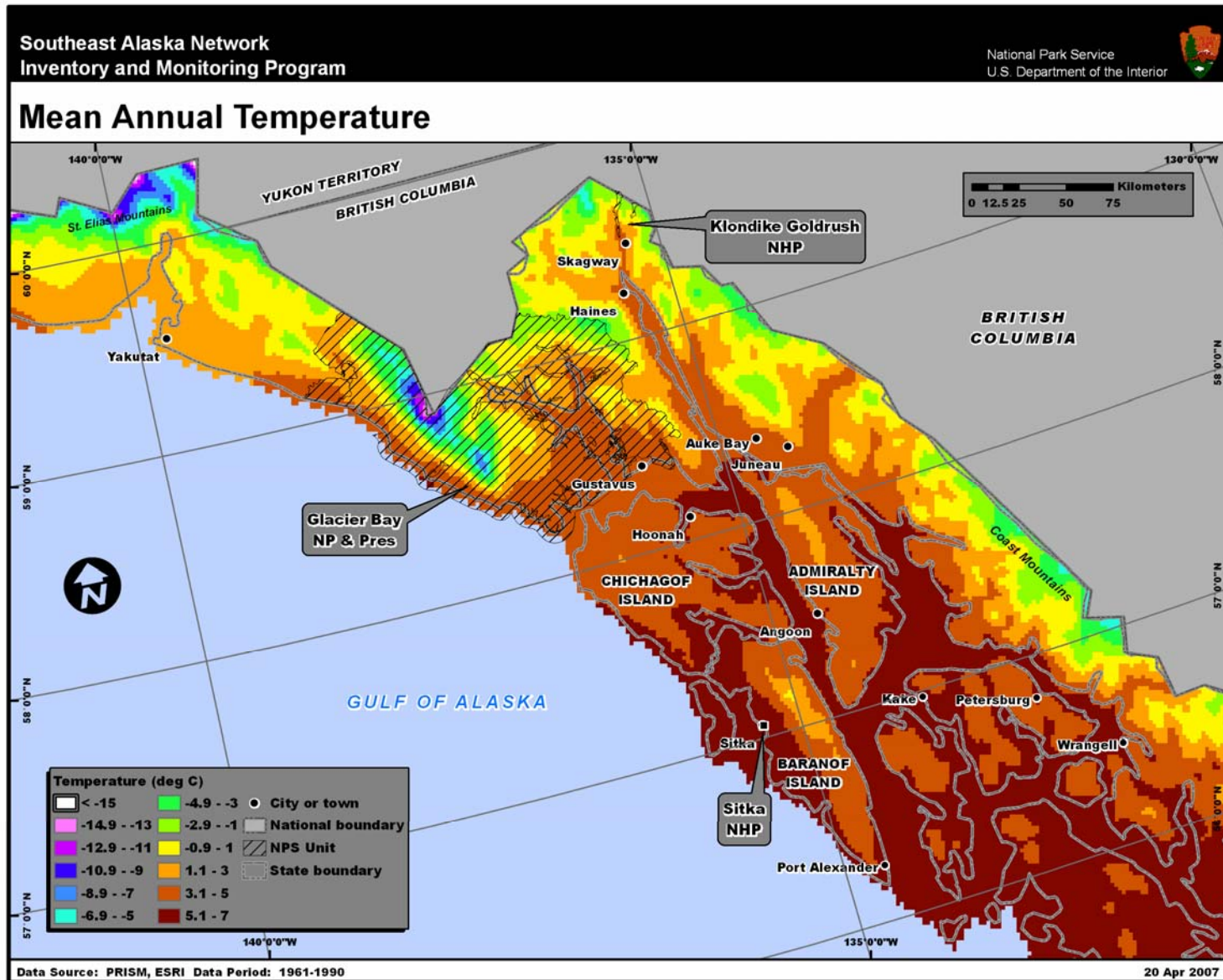
Figure 2.3. Mean annual temperature, 1961-1990, for the SEAN.
