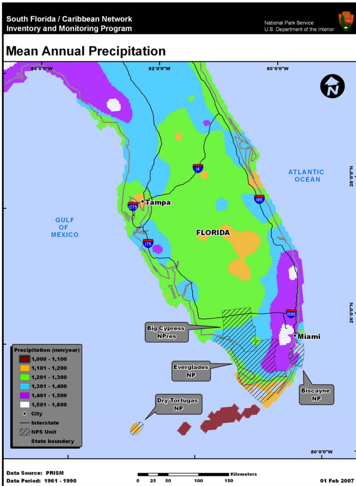
Figure 2.1. Mean annual precipitation, 1961-1990, for the SFCN.
