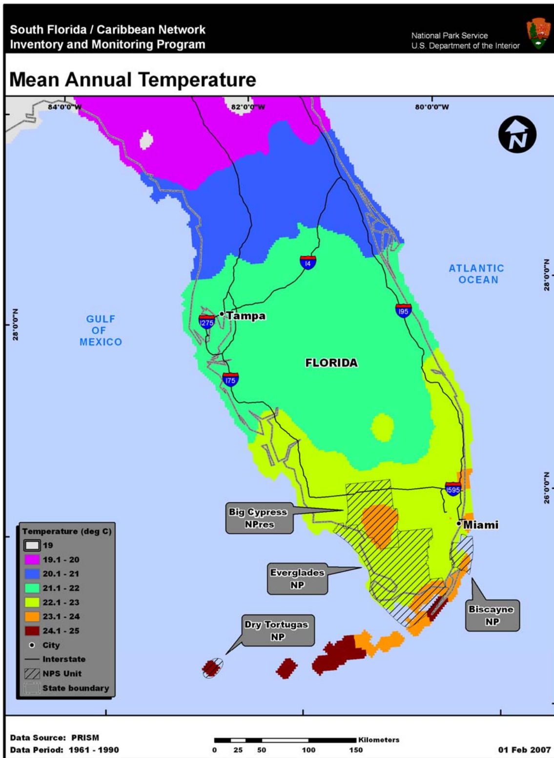
Figure 2.4. Mean annual temperature, 1961-1990, for the SFCN.
