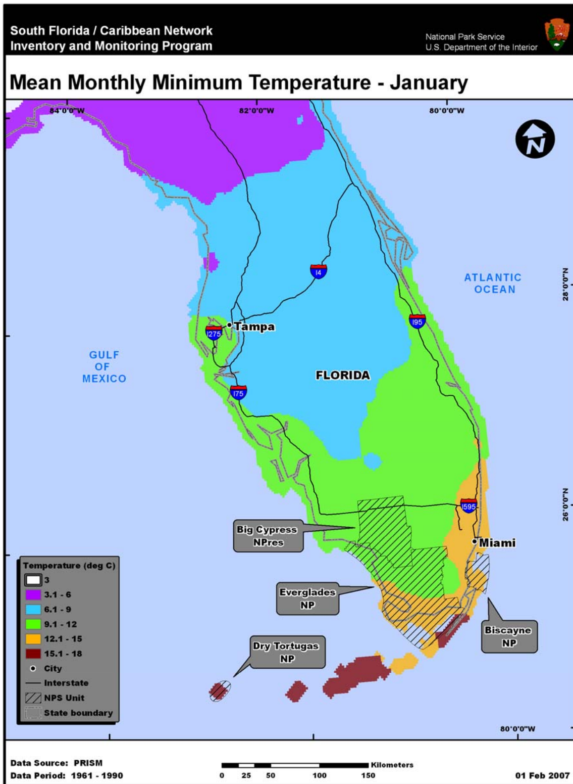
Figure 2.5. Mean January minimum temperature, 1961-1990, for the SFCN.
