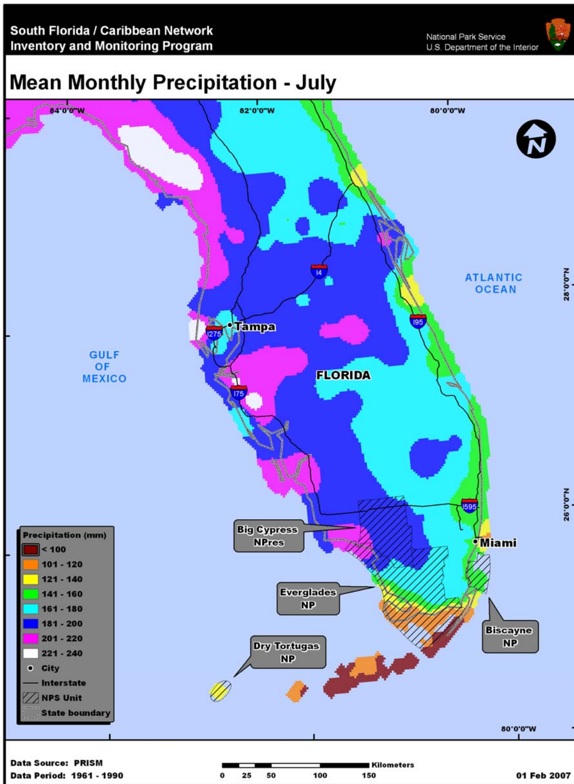
Figure 2.3. Mean July precipitation, 1961-1990, for the SFCN.
