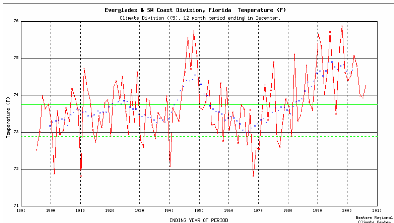
Figure 2.8. Temperature time series, 1895-2005, for southern Florida, including twelve-month average temperature (ending in December) (red), 10-year running mean (blue), mean (green), and plus/minus one standard deviation (green dotted).
