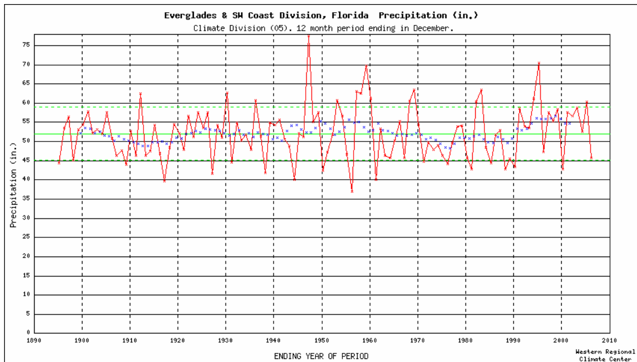
Figure 2.7. Precipitation time series, 1895-2005, for southern Florida, including twelve-month precipitation (ending in December) (red), 10-year running mean (blue), mean (green), and plus/minus one standard deviation (green dotted).
