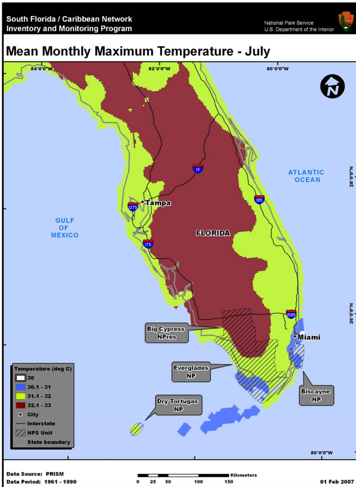
Figure 2.6. Mean July maximum temperature, 1961-1990, for the SFCN.
