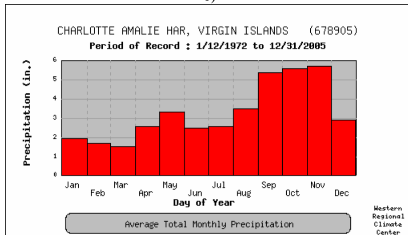
Figure 2.2. Mean monthly precipitation at selected stations in the SFCN. Locations include Tamiami Trail 40 Mi. Ben (a) near EVER, Key West Airport (b) east of DRT0 (b), and Charlotte Amalie Har. (c) near BUIS and SARI.
